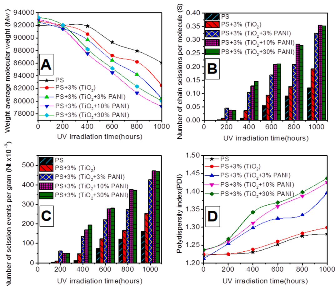
Fig. 5. A) Weight average molecular weight ( \bar{M}_w ), B) Number of chain scissions per molecule (S), C) number of scission events per gram ( N_t ) and D) Polydispersity index (PDI) of PS and PS-composite under different UV irradiation time.
